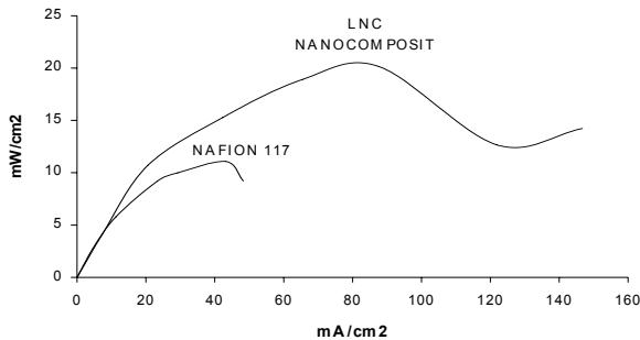
Figure 13. Power efficiency curve of PEM fuel cell utilizing LNC composite membrane and nafion membrane
