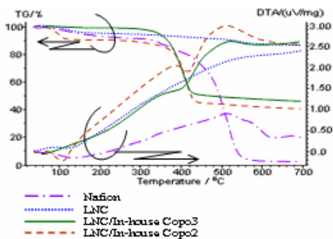
Figure 7. DTA/TG data of LNC nano composites with various emulsion polymers
