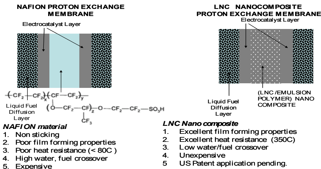
Figure 11. Comparison between LNC Nano Composite PEM and Nafion PEM in PEM FC
