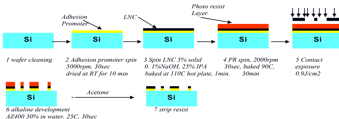
Figure 9 Micro pattern imaging process of LNC
