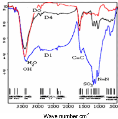
Figure 4 FtIR spectrums of D0, D1, and D4
