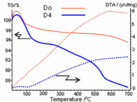
Figure 6. DTA/TG data of LNC (D4) and \text{D}_0
