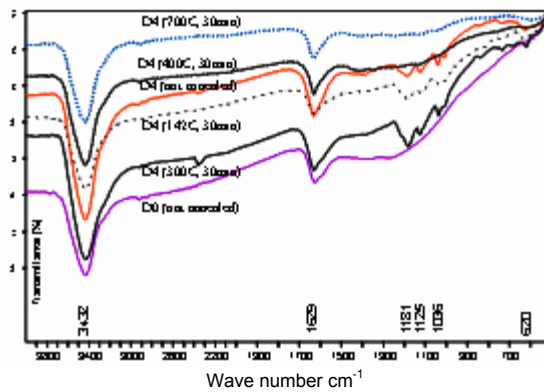
Figure 5 FtIR spectrum of LNC (D4) annealed at various temperature
