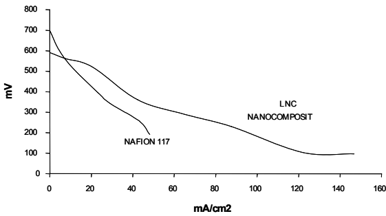
Figure 12 V-I characteristic curves of the PEM made out of LNC Nano Composite compared to that of commercial Nafion 117
