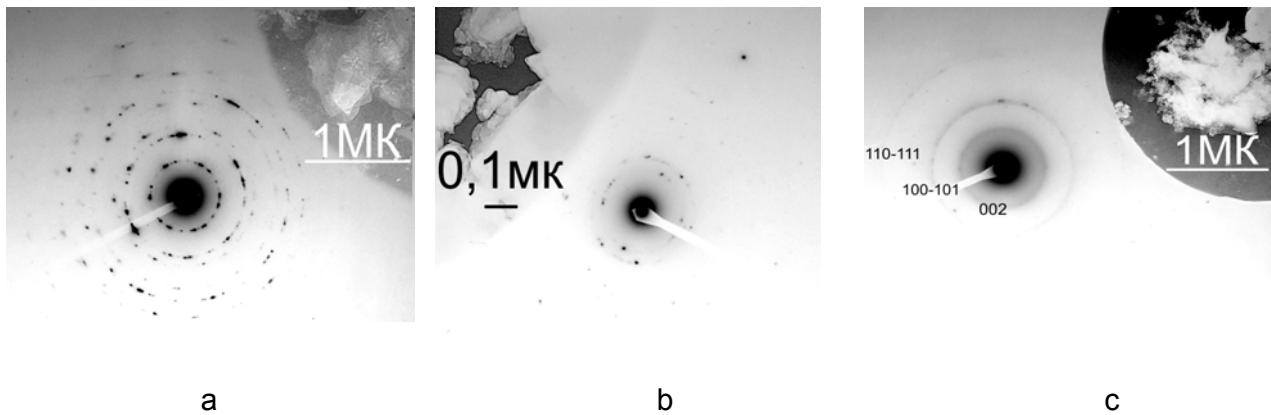
Fig.1. Electron microscopic pictures and electron diffraction of modified particles quartz.
