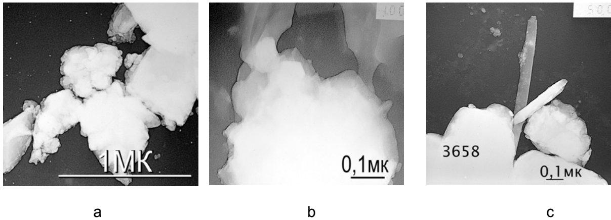
Fig.2. Electron microscopic pictures at different stages of formation of a modified layer of a quartz particle.
